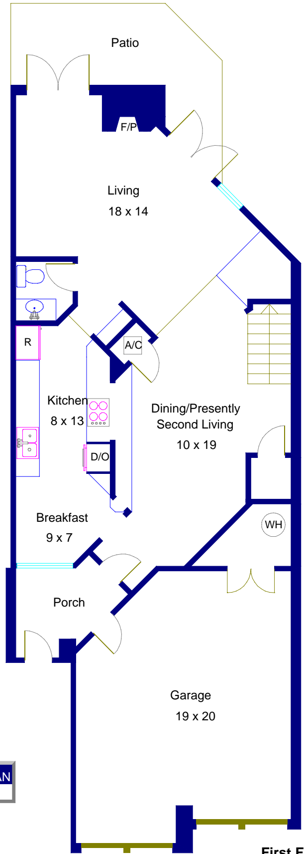
First Floor
